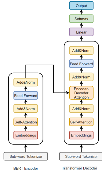
Figure 1: Construction of NMT engine with pre-trained model BERT.
