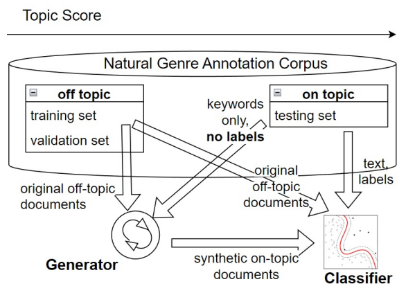
Figure 1: Experimental workflow
